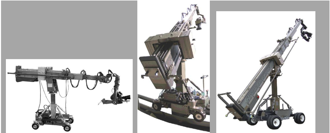
HYDRASCOPE: 15', 20' 32' ( Waterproof Telescoping Crane Arm )
